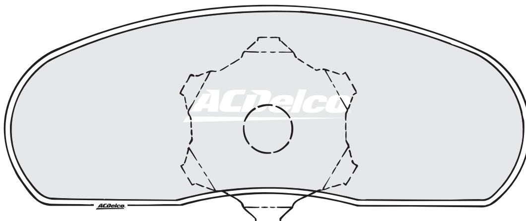
ACD6 (13.1mm) INNER Chrysler Holden Leyland (BLMC) Toyota
