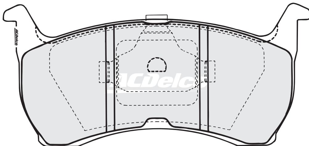
ACD1108 (13.2mm) INNER FORD (AUST.)
