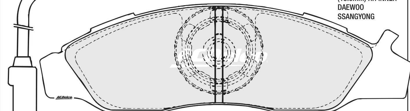
ACD1337 (16.5mm) RH OUTER DAEWOO SSANGYONG
