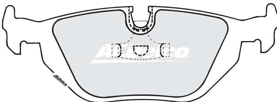
ACD1245 (17.0mm) INNER BMW
